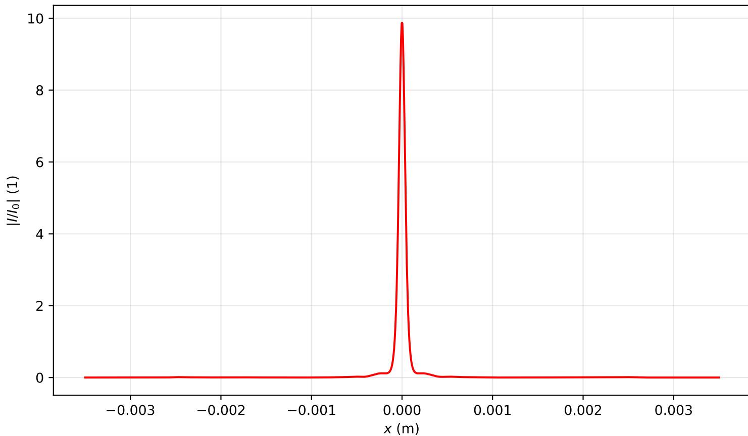
Intensity profile I(x, y = 0, z = 1.433)/I_0 , P_{in}=5.0P_{cr} , artificial time
